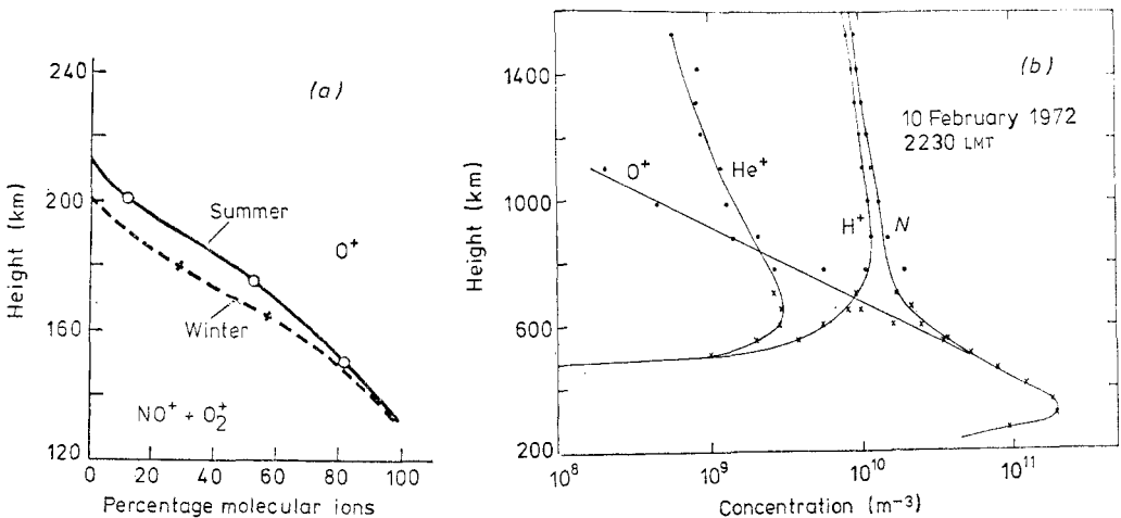
Figure 13. (a) Relative concentrations of ions with height: transition from molecular ions [NO^+ + O_2^+] to atomic ions [O^+] observed at St Santin (from Waldteufel 1970). (b) Relative concentrations of ions with height: O^+ , He^+ , H^+ at Arecibo. The concentration of electrons ( N ) is also shown (from Hagen and Hsu 1974).
