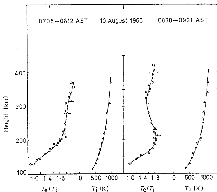
Figure 10. T_e/T_i measured from ion spectrum ( \circ ) and plasma lines ( \bullet ). T_i from ion component ( \Delta ).
