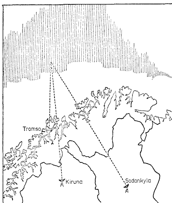
Figure 28. EISCAT stations. UHF system: 933 MHz transmitter at Tromsø, receivers at Tromsø, Kiruna and Sodankylä. VHF system: 224 MHz transmitter at Tromsø, receiver at Tromsø. Tromsø–Sodankylä = 390.5 km, Tromsø–Kiruna = 197.6 km, Kiruna–Sodankylä = 268.6 km.
