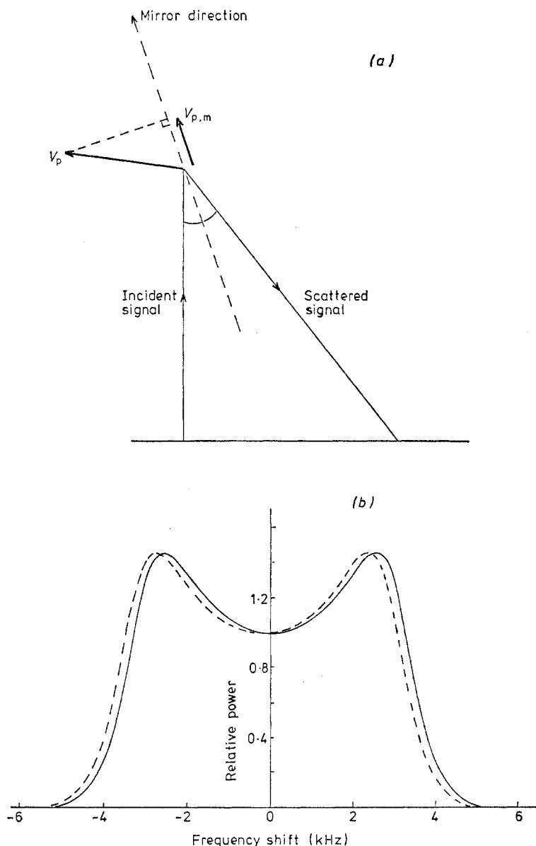
Figure 14. (a) The mirror direction for a bistatic system, showing the component of plasma drift velocity ( V_{p,m} ) measured by such a system. (b) Ion spectrum for zero plasma velocity (—) and for a plasma velocity of 100 m s ^{-1} in the mirror direction (---). T_e = 1500 K, T_i = 1000 K, M_i = 16 ( O^+ ), \lambda = 1 m.
