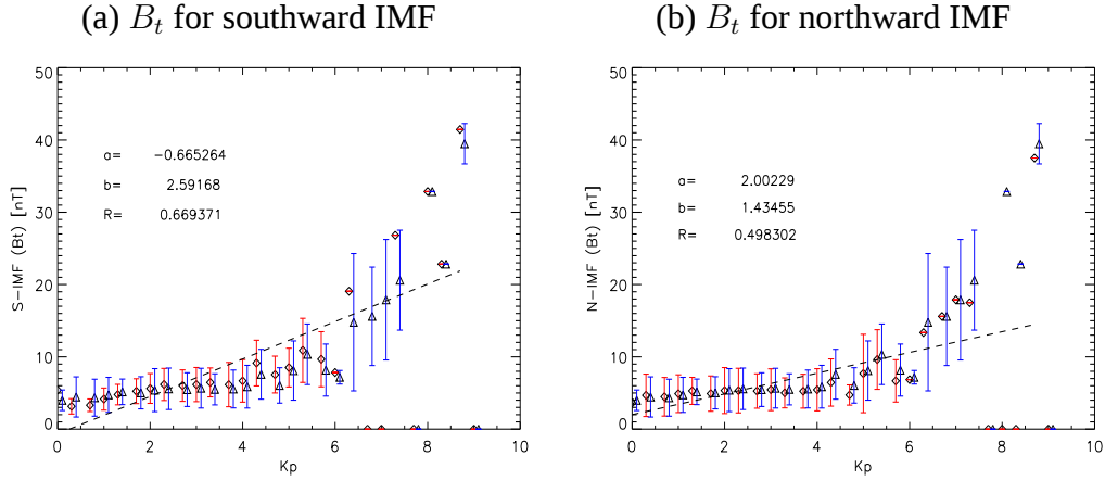
Figure 3.5: K_p (horizontal axis) versus the IMF projection onto the YZ_{gsm} plane ( B_t ). (a) B_t (intensity) for southward IMF (3-hour averaged, fluctuations during 3-hour period are not considered) ( \diamond with red error bar), (b) B_t for northward IMF (same style as (a)), and the mark \triangle with blue error bar represents B_t for arbitrary orientations of IMF. As shown in the figures, intensity of the IMF seems not to be related to K_p independent of the IMF orientation, except for higher K_p , e.g. K_p > 6 .
