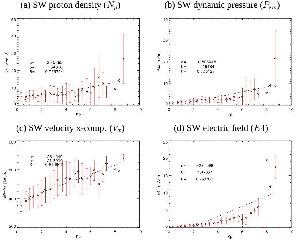
Figure 3.4: K_p (horizontal axis) versus the solar wind parameters. The solar wind parameters shown in the panels (from the top, left to right) are (a) solar wind proton density ( N_p ), (b) solar wind dynamic pressure ( P_{sw} ), (c) solar wind velocity x-component ( V_x ), (d) solar wind electric field ( E4 ). The 3-hour averaged ACE data are utilized and K_p -related averages and standard deviations (SD) of the solar wind parameters are derived. The data are fitted to the linear model, y = a + bx , and the linear Pearson correlation coefficients ( R ) are computed.
