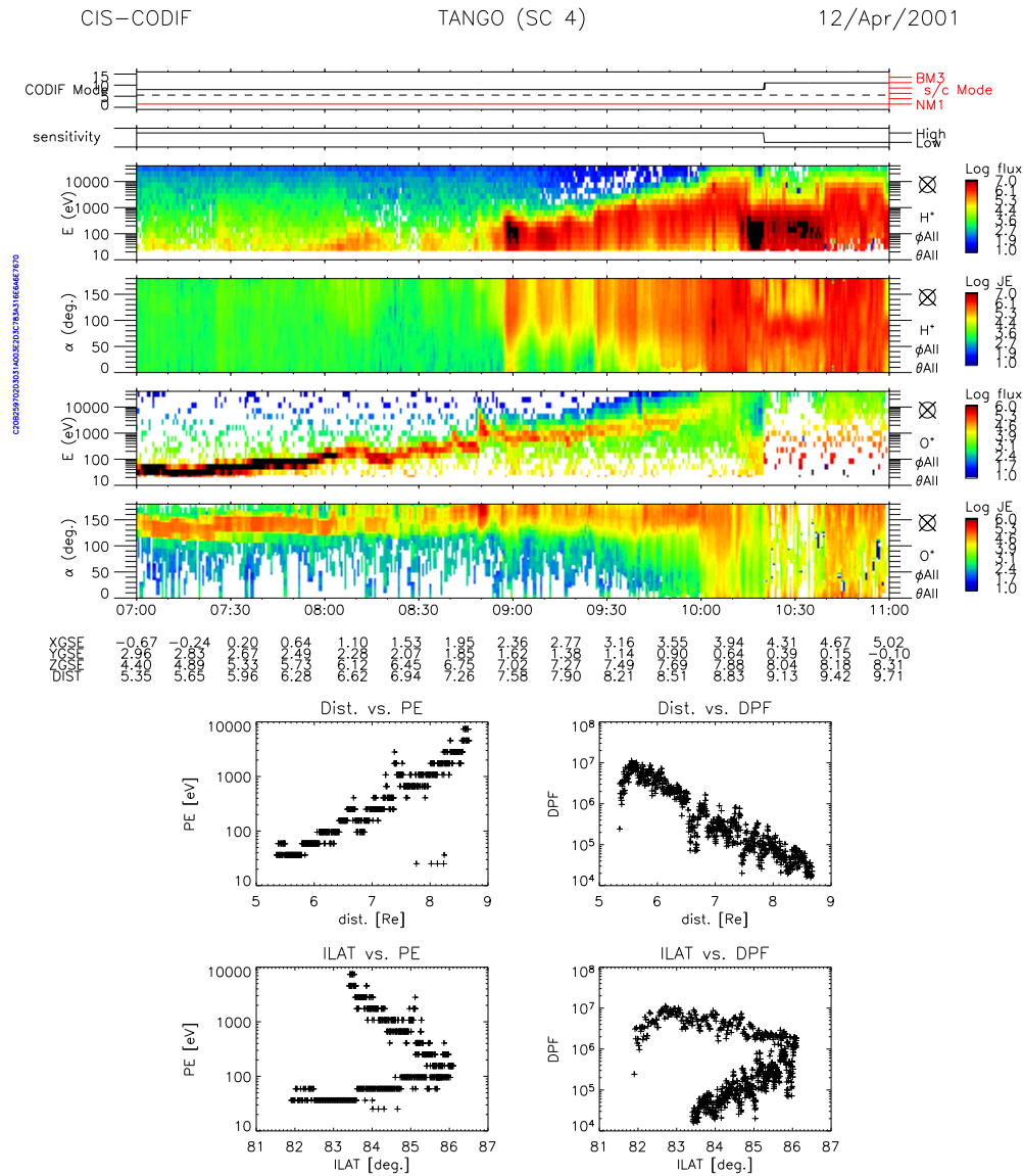
Figure 3.1: (Upper) A sample data provided by the Cluster CIS/CODIF instrument. The 5th and 6th panels, from the top, show time-energy spectrogram and time-pitch angle distributions of O^+ . As seen in the panels, field-aligned upgoing O^+ with narrow energy band were observed continually in long time period, i.e. from 07:00 UT to 10:00 UT. (Bottom) The PE and MDPF distributions as functions of geocentric distance and ILAT are also shown. The data set is the same as the above.
