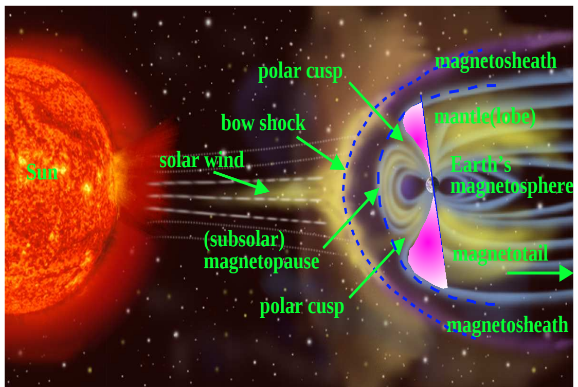
Figure 1.1: Schematic diagram of the Sun, Earth's magnetosphere and the Sun-Earth interaction. The region focused on in this thesis is emphasized. Several key terms and the corresponding locations are also displayed. Original picture from NASA (non-protected by copyright law unless noted).
