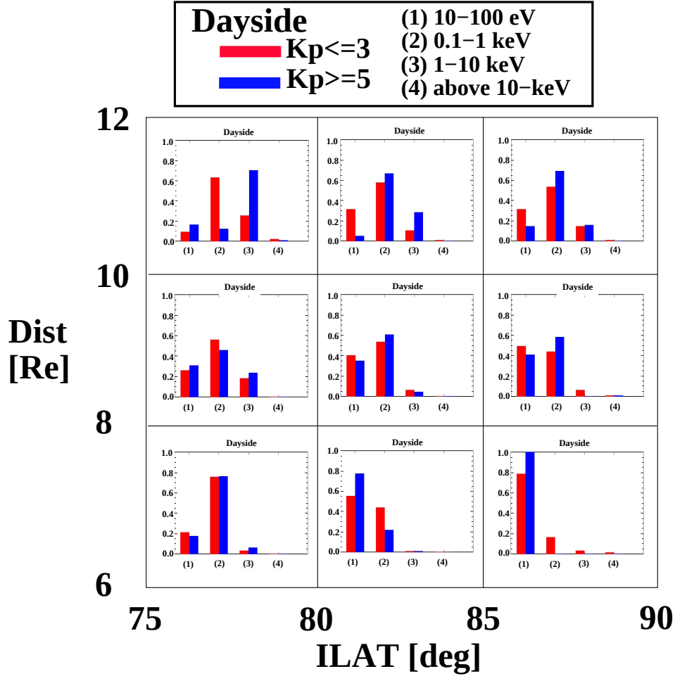
Figure 3.2: The occurrence rates of different PE levels in the dayside high-altitude and high-latitude region. The whole region is divided into 2R_E \times 5^\circ subregions, and the pairs of bars denote different K_p conditions (red: K_p \leq 3 , blue: K_p \geq 5 ) and stand in a horizontal line, ordered from the left-hand side, (1) 10 \leq PE < 100 eV, (2) 0.1 \leq PE < 1.0 keV, (3) 1.0 \leq PE < 10.0 keV, and (4) PE \geq 10.0 keV.
