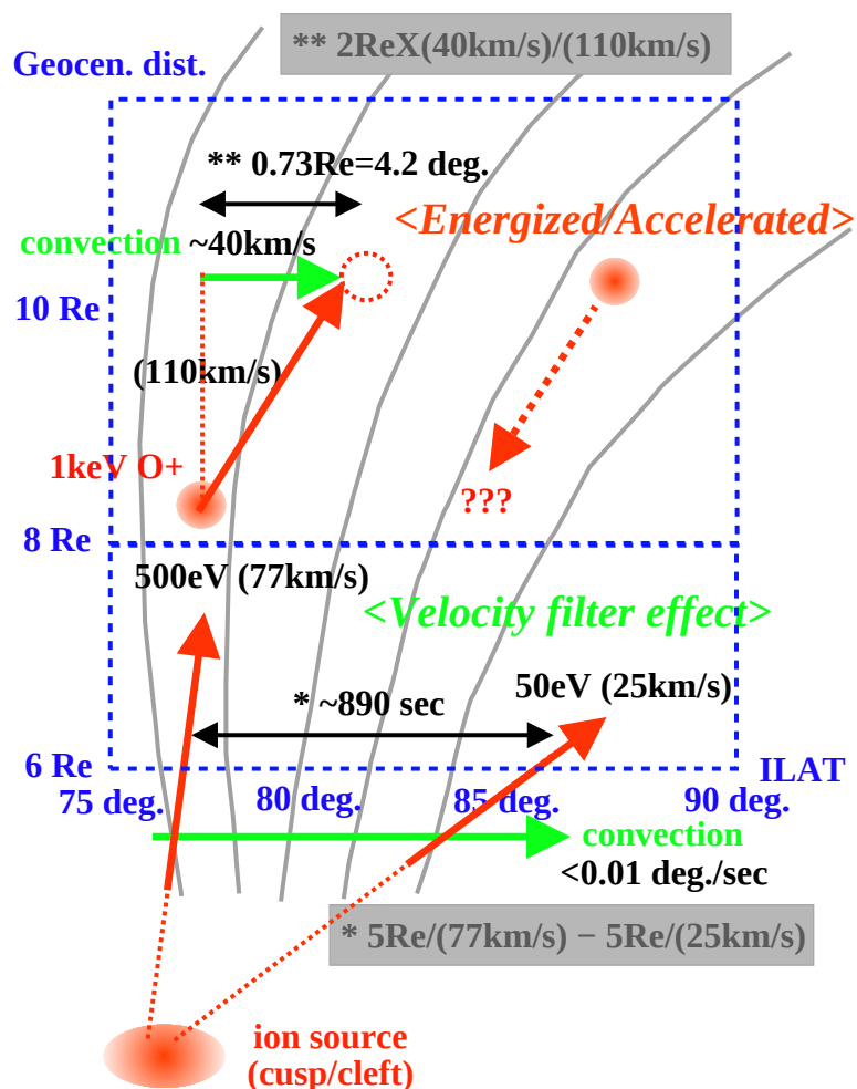
Figure 3.3: Not-scaled schematic interpreting Fig. 3.2. This sketch shows that latitudinal distribution of outflowing O^+ observed below 8 R_E geocentric distance can be explained by velocity filter effect, while the distribution above 10 R_E geocentric distance cannot be explained by the velocity filter effect only. Thus we suggest that additional energization/acceleration takes place at such high altitudes and high latitudes. Note that K_p dependence is not taken into account in this sketch.
