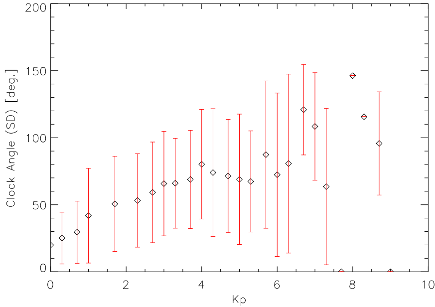
Figure 3.6: K_p (horizontal axis) versus the standard deviation (SD for 3-hour average of ACE data) on IMF clock angle ( \theta ). The SDs are averaged over a given K_p value.
