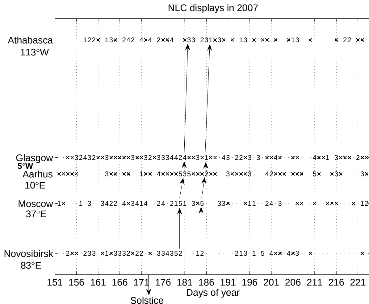
Figure 3. All NLC displays observed in Novosibirsk, Moscow, Aarhus, Port Glasgow and Athabasca in 2007. The numbers stand for the maximal brightness of NLCs (on a five point scale) on a given night. Crosses are nights with bad weather. Dots are an absence of NLCs on clear nights.
