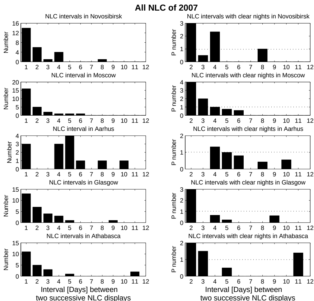
Figure 8. Histograms of time intervals between two successive NLC displays observed from Novosibirsk, Moscow, Aarhus, Port Glasgow and Athabasca in 2007.
