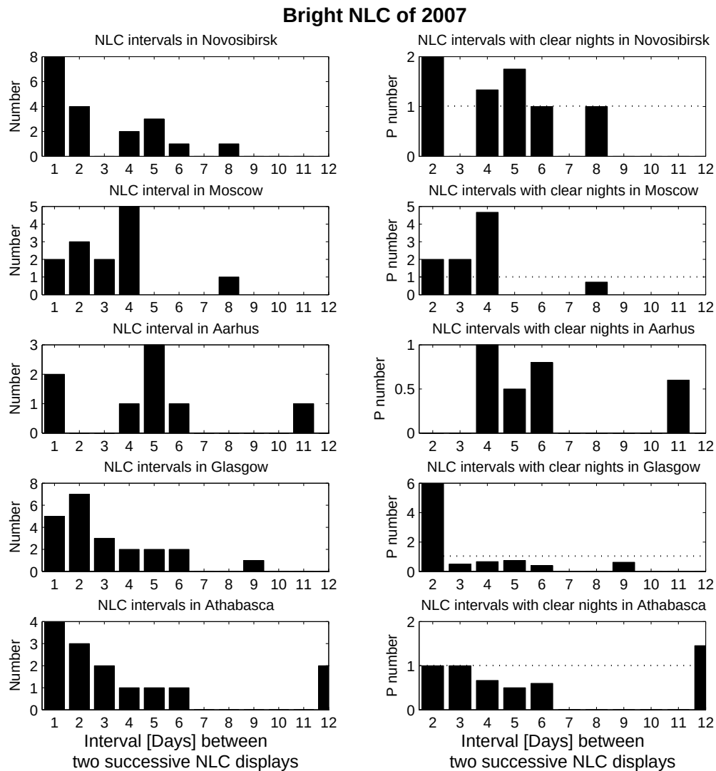
Figure 9. Histograms of time intervals between two successive bright and/or extended NLC displays observed from Novosibirsk, Moscow, Aarhus, Port Glasgow and Athabasca in 2007.
