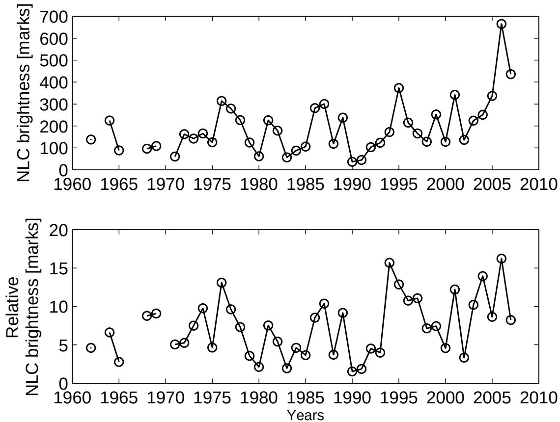
Figure 5. The upper panel: yearly variation of the NLC brightness in Moscow. The lower panel: time series of normalized NLC brightness (normalized by the number of clear weather nights) in Moscow.
