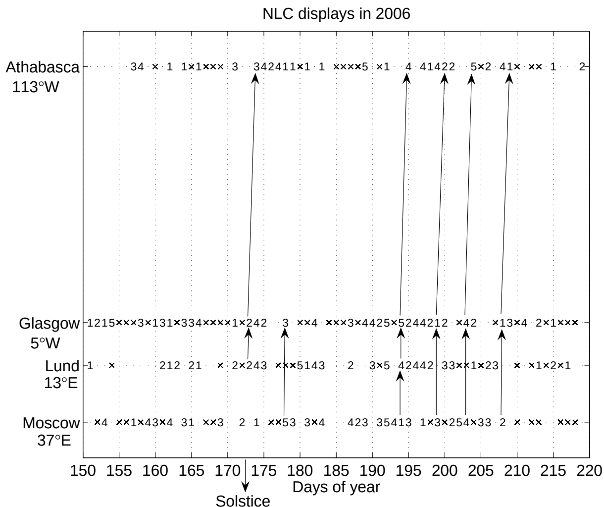
Figure 2. All NLC displays observed in Moscow, Lund, Port Glasgow and Athabasca in 2006. The numbers stand for the maximal brightness of NLCs (on a five point scale) on a given night. Crosses are nights with bad weather. Dots are an absence of NLCs on clear nights.
