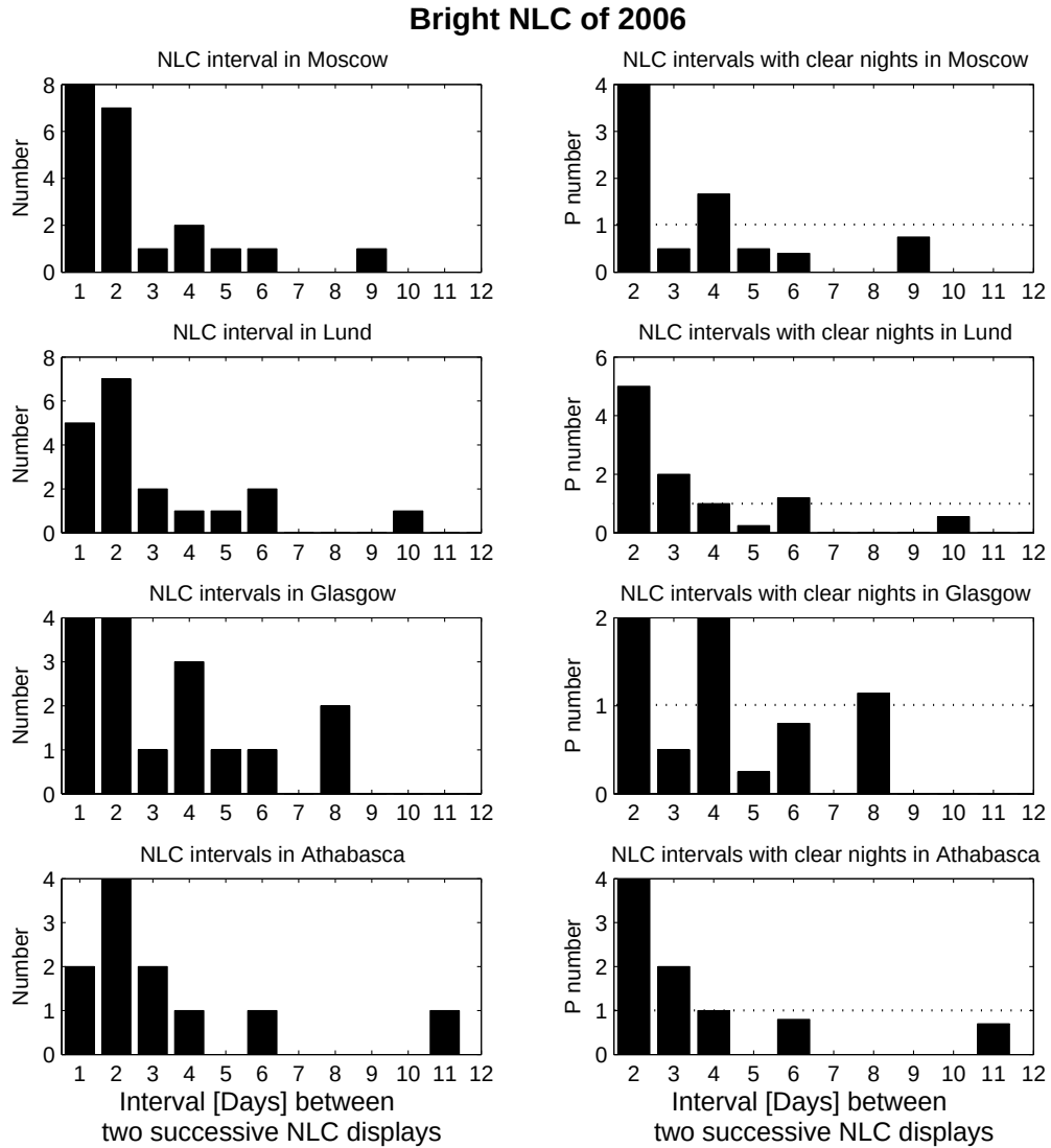
Figure 7. Histograms of time intervals between two successive bright and/or extended NLC displays observed from Moscow, Lund, Port Glasgow and Athabasca in 2006.
