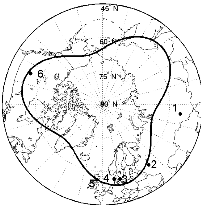
Figure 1. Map demonstrating locations of NLC cameras in 2006 and 2007: 1 – Novosibirsk, Russia ( 54^\circ\text{N}52' ; 83^\circ\text{E}06' ); 2 – Moscow, Russia ( 56^\circ\text{N}00' ; 37^\circ\text{E}29' ); 3 – Lund, Sweden ( 55^\circ\text{N}43' ; 13^\circ\text{E}13' ); 4 – Aarhus, Denmark ( 56^\circ\text{N}10' ; 10^\circ\text{E}12' ); 5 – Port Glasgow, Scotland ( 55^\circ\text{N}56' ; 04^\circ\text{W}41' ); 6 – Athabasca, Canada ( 54^\circ\text{N}44' ; 113^\circ\text{W}19' ). The thick curve represents schematically the 2-day planetary wave with zonal wavenumber 3 (see the text).
