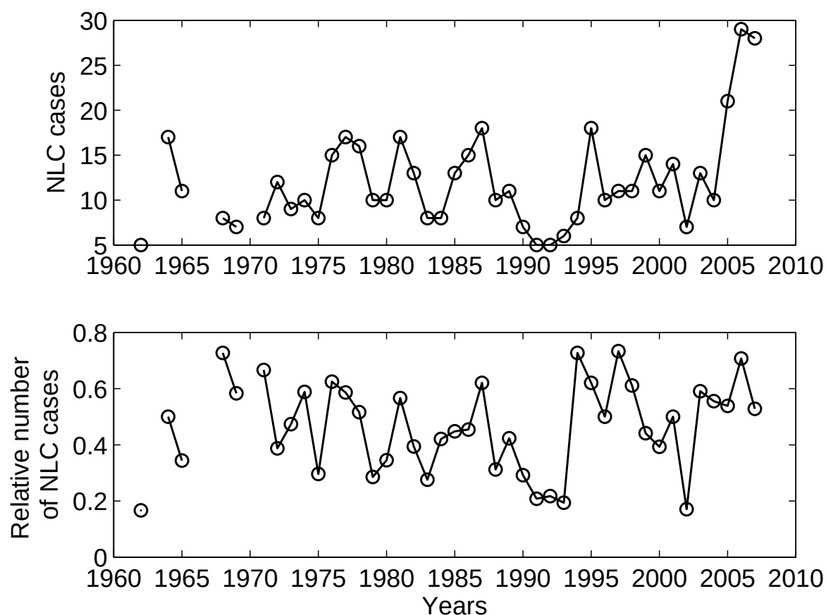
Figure 4. The upper panel: yearly variation in the total number of nights with NLC in Moscow. The lower panel: time series of normalized NLC frequency (normalized by the number of clear weather nights) in Moscow.
