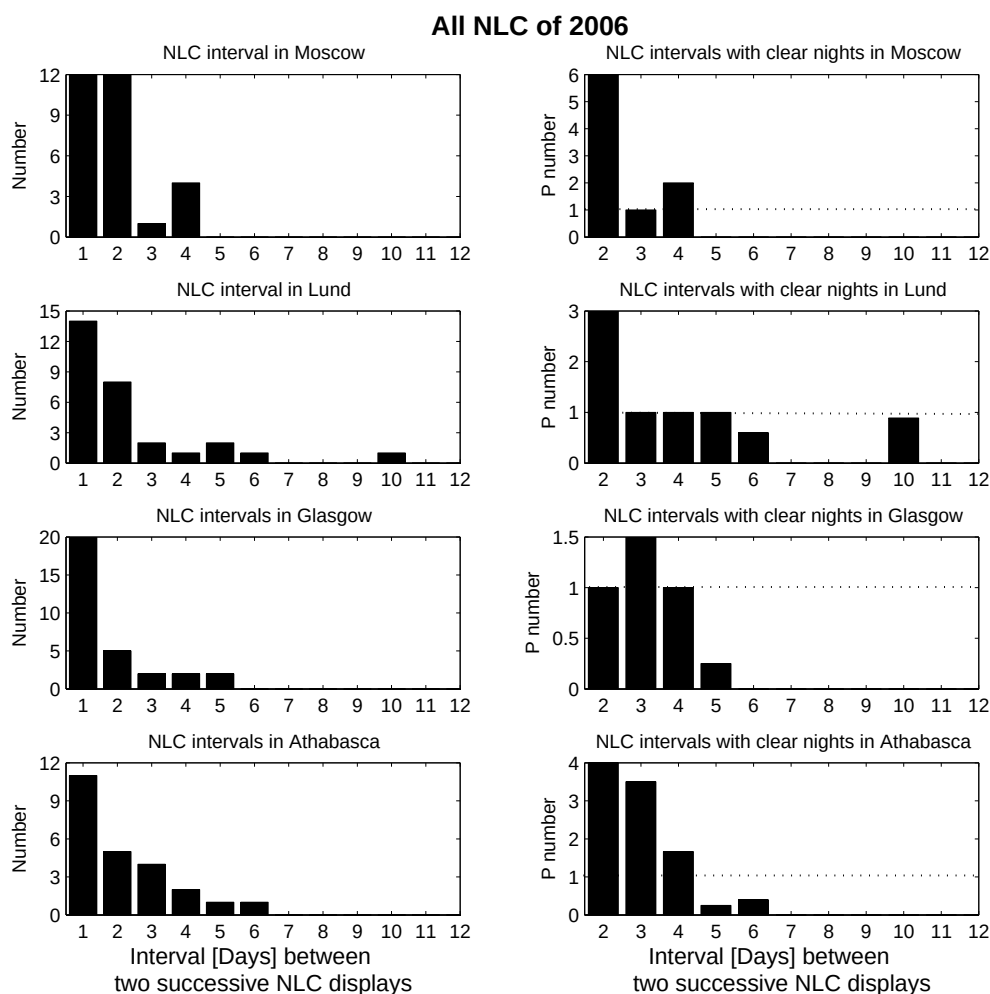
Figure 6. Histograms of time intervals between two successive NLC displays observed from Moscow, Lund, Port Glasgow and Athabasca in 2006.
